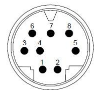
Mini-DIN 8P
